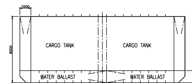
MIDSHIP SECTION
