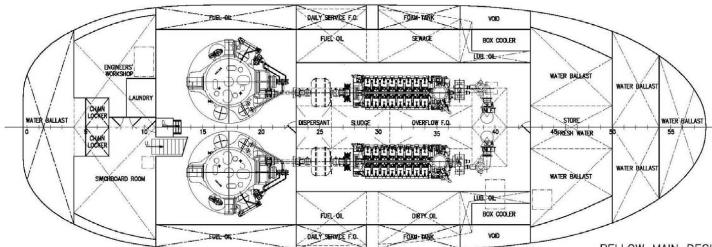
BELLOW MAIN DECK
