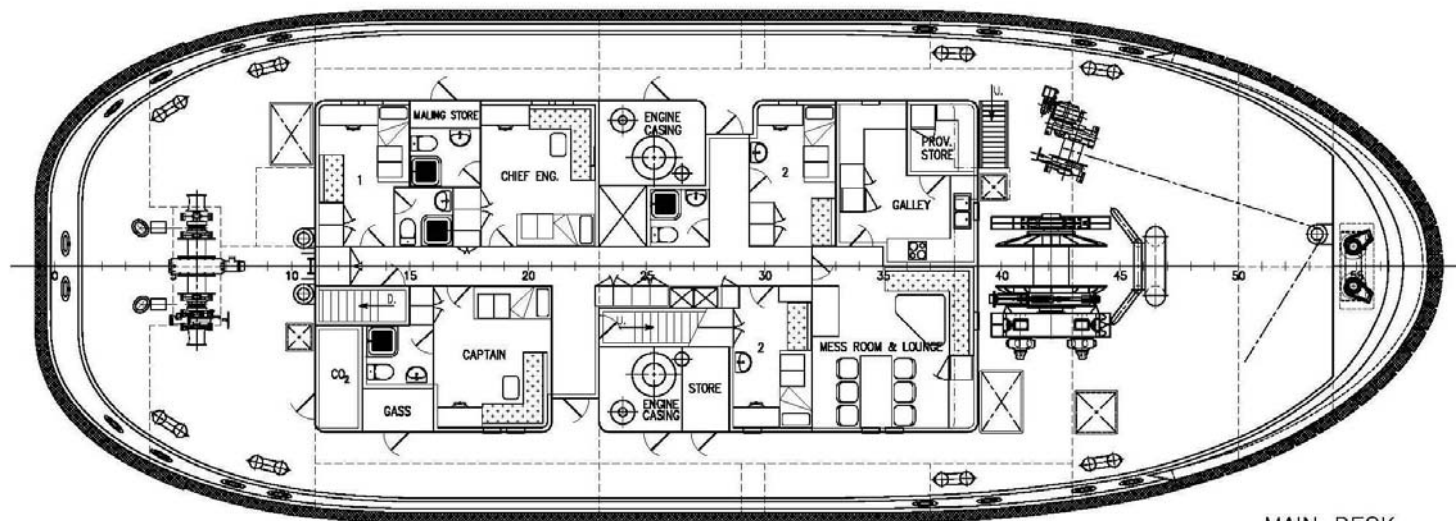
MAIN DECK
